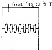
FIG. 222. STRAIGHT STITCH BELT LACE.
